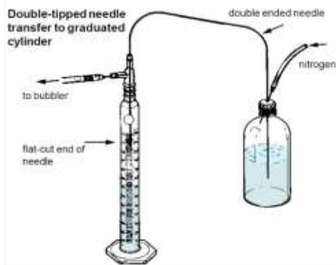
Fig. 3B. Double-tipped needle transfer to graduated cylinder
