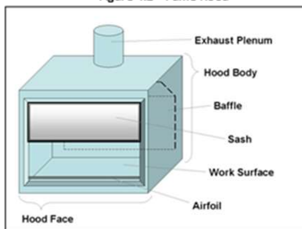
Figure 4.2 – Fume Hood
