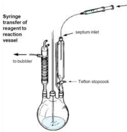
Fig. 2C Syringe transfer of reagent to reaction vessel
