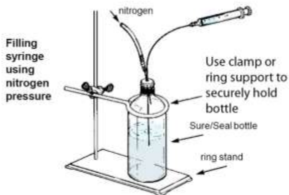
Fig. 2A. Filling syringe using nitrogen pressure
