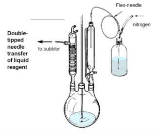
Fig. 2 Double-tipped needle transfer of liquid reagent
