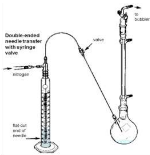
Fig. 3C. Double-ended needle transfer with syringe valve
