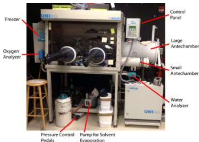
Figure 4.3 – Glovebox
