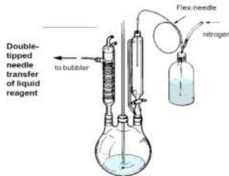
Fig. 3A. Double-tipped needle transfer of liquid reagent
